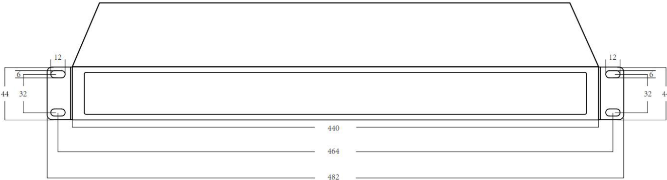
Rack mounting ears
