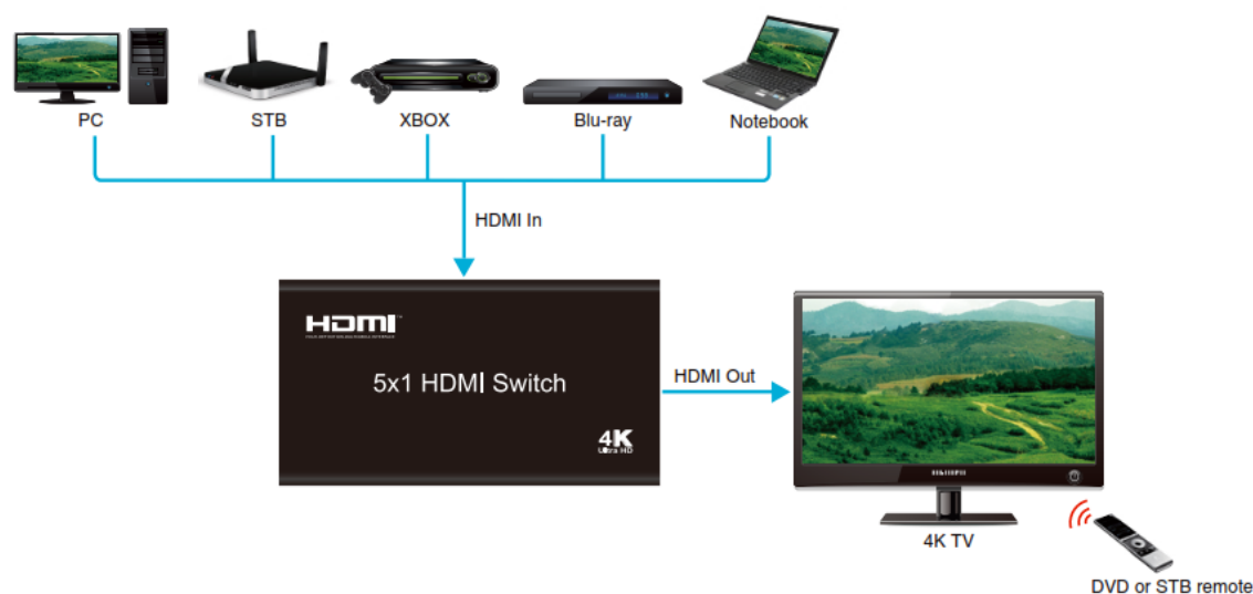
Connection Diagram
